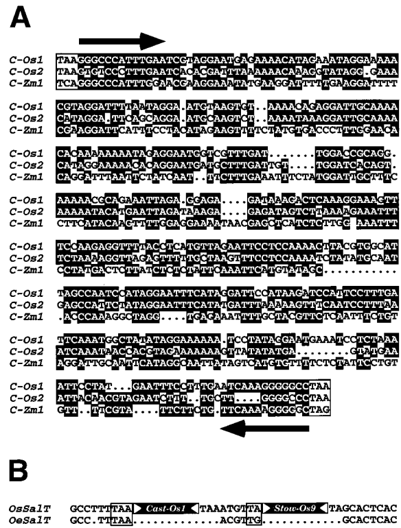
FIG. 2. (A) Multiple sequence alignments of Castaway ( C ) family members. Solid arrows indicate the position of TIRs, and boxed regions indicate the putative target site of insertion. Dotted lines are gaps. (B) Insertion polymorphism between the 5'-flanking region of the Salt gene in O. sativa ( OsSalt ) and O. eichingeri ( OeSalt ). This polymorphism is due to the insertion of two elements, Castaway-Os1 ( Cast-Os1 ) and Stowaway-Os9 ( Stow-Os9 ). The boxed region indicates the putative target site sequence. Dotted lines are gaps.
